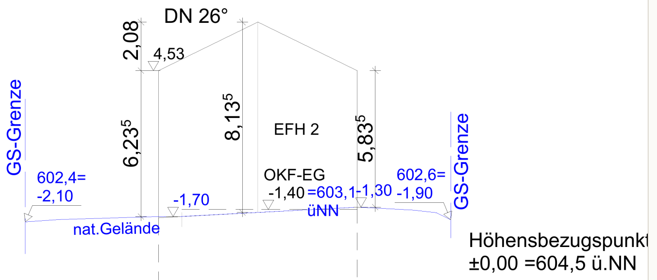
A4, Nord-West (Giebel hofseitig)
